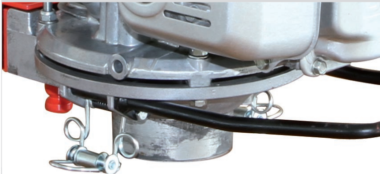
WEIGHT OPTIMISED FLANGE + ARRESTMENT OF THE CLAMP
